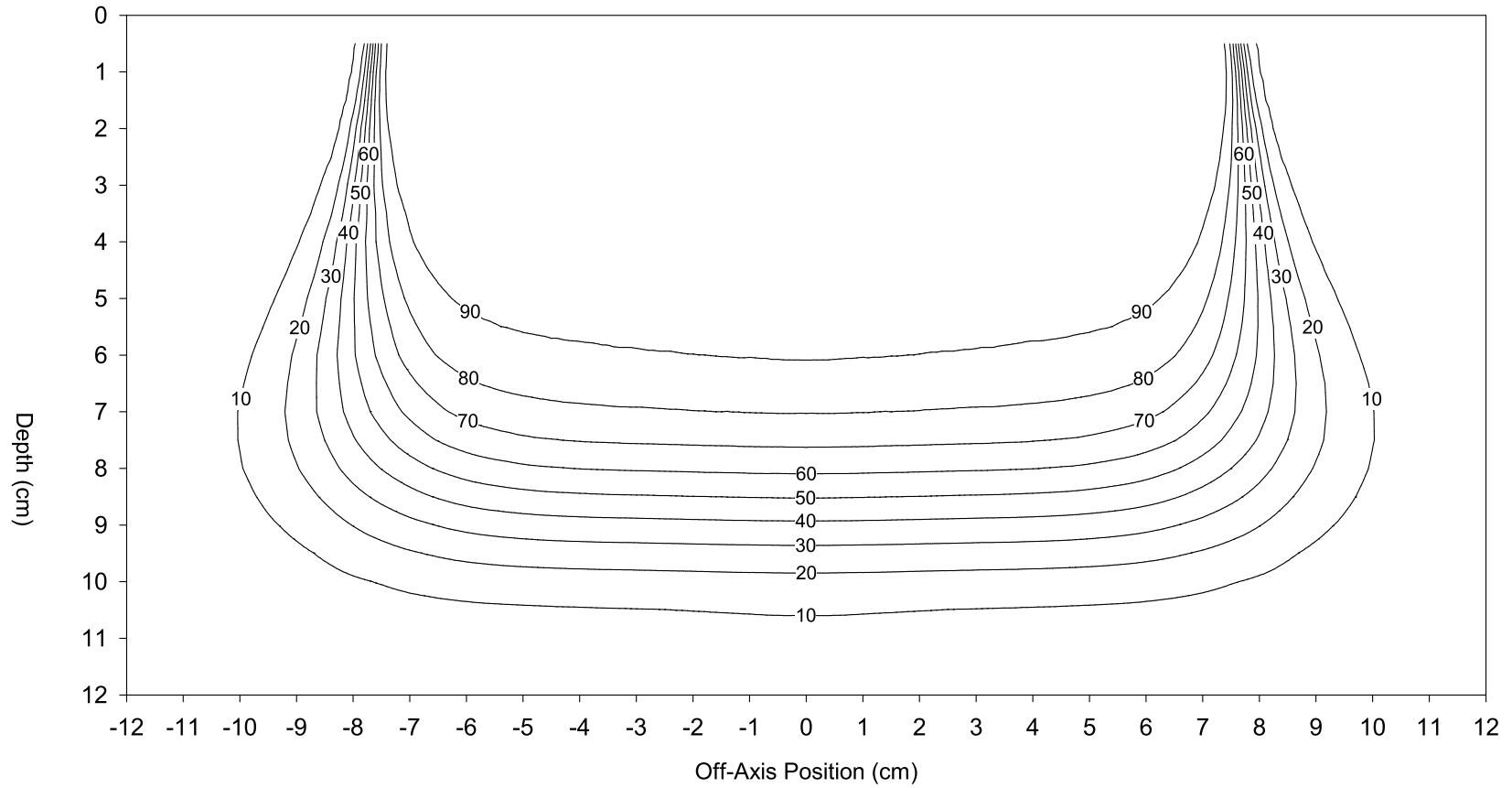
Configuration 3 - 20 MeV, Water, 100-cm SSD
