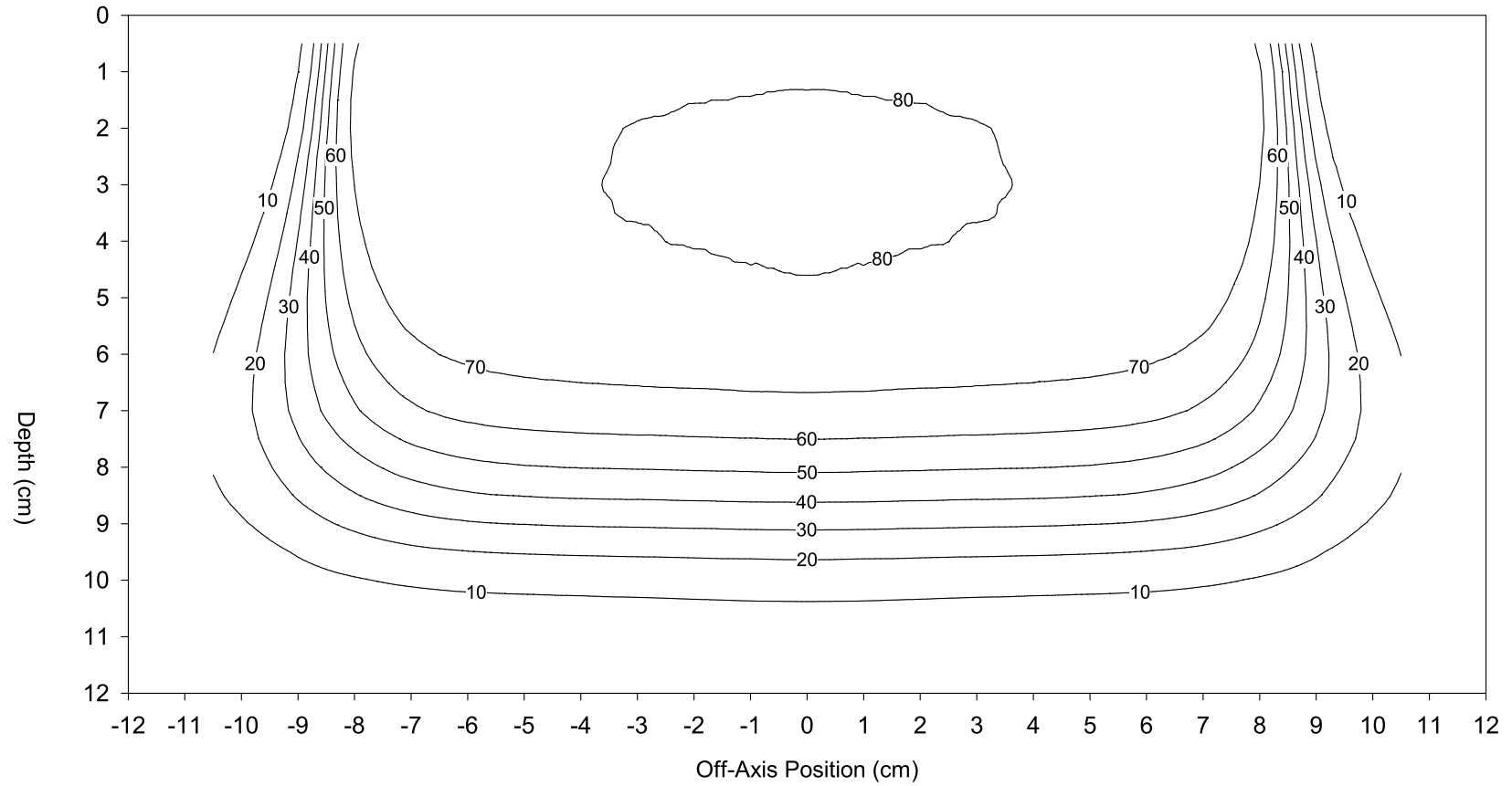
Configuration 4 - 20 MeV, Water, 110-cm SSD
