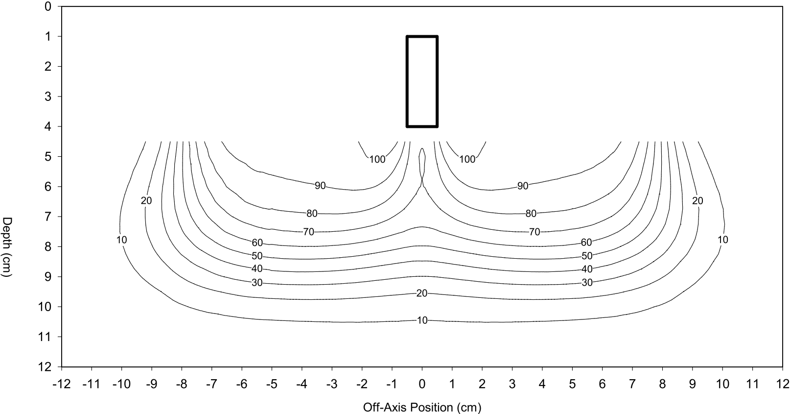
Configuration 10 - 20 MeV, Vertical Bone Slab, 100-cm SSD
