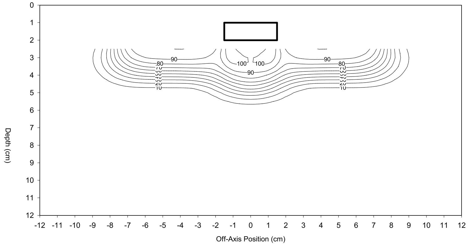
Configuration 5 - 9 MeV, Horizontal Air Slab, 100-cm SSD
