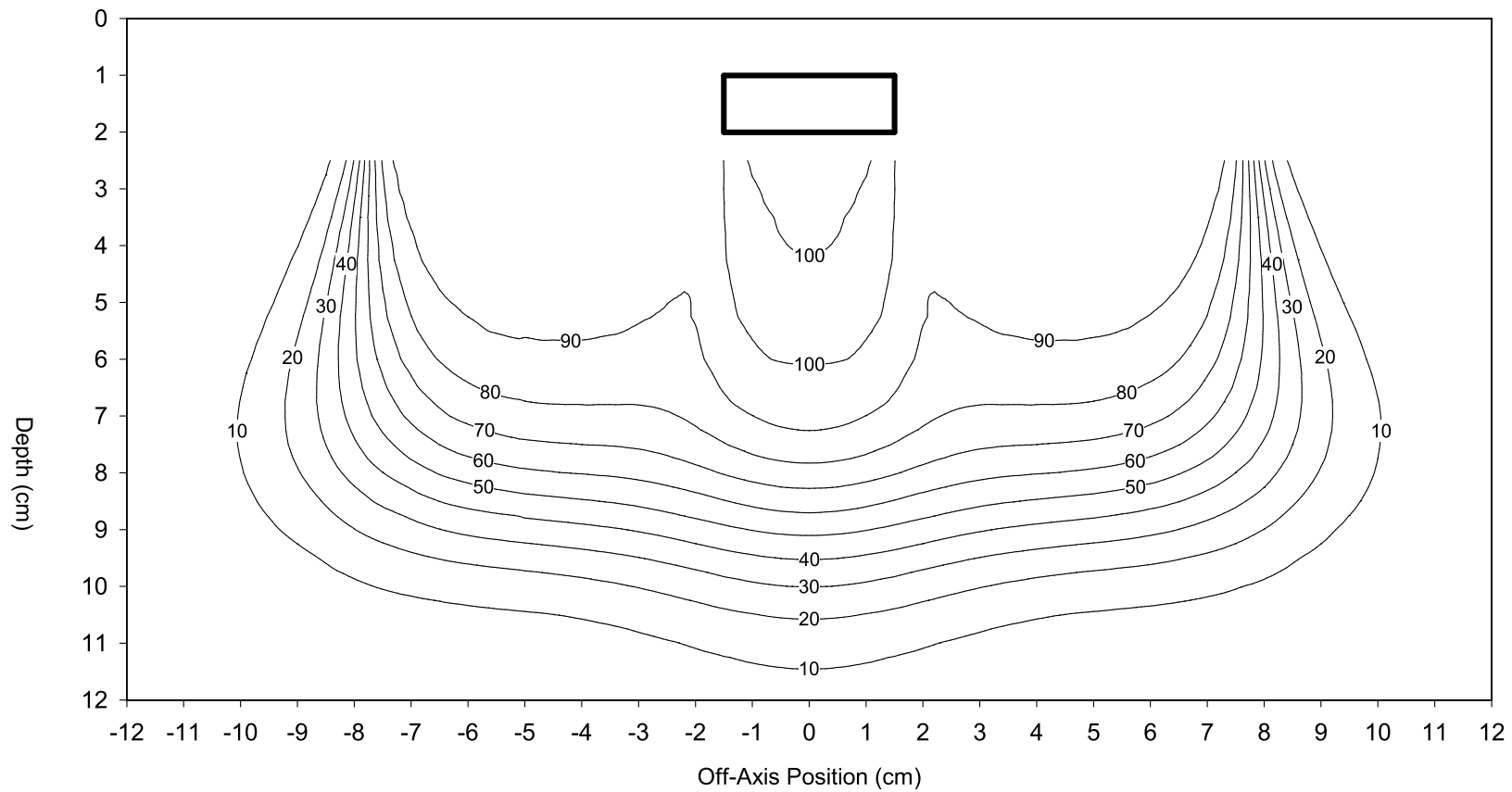
Configuration 6 - 20 MeV, Horizontal Air Slab, 100-cm SSD
