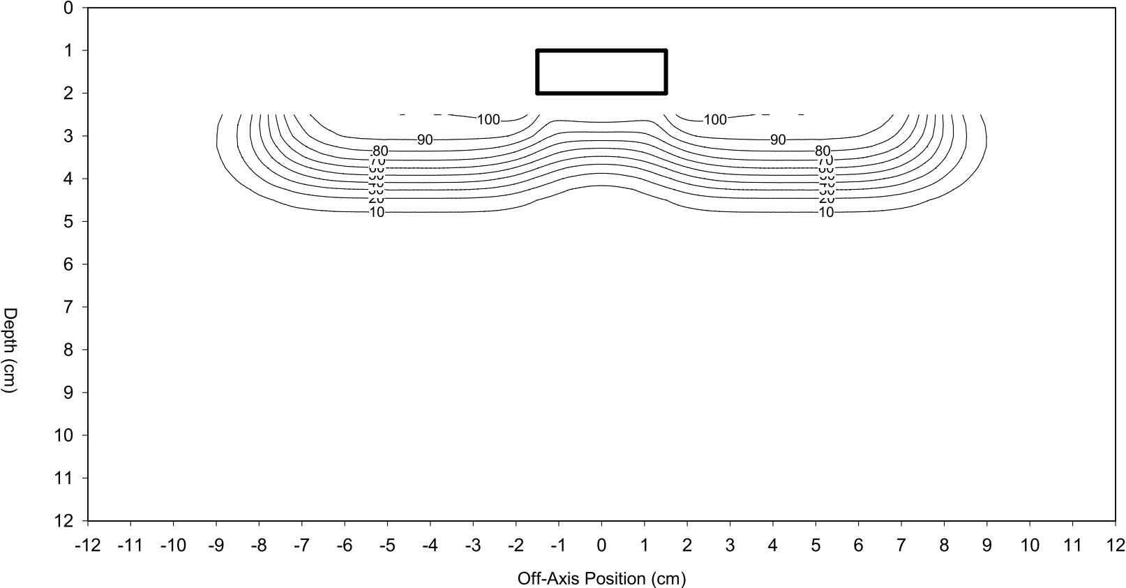
Configuration 8 - 9 MeV, Horizontal Bone Slab, 100-cm SSD
