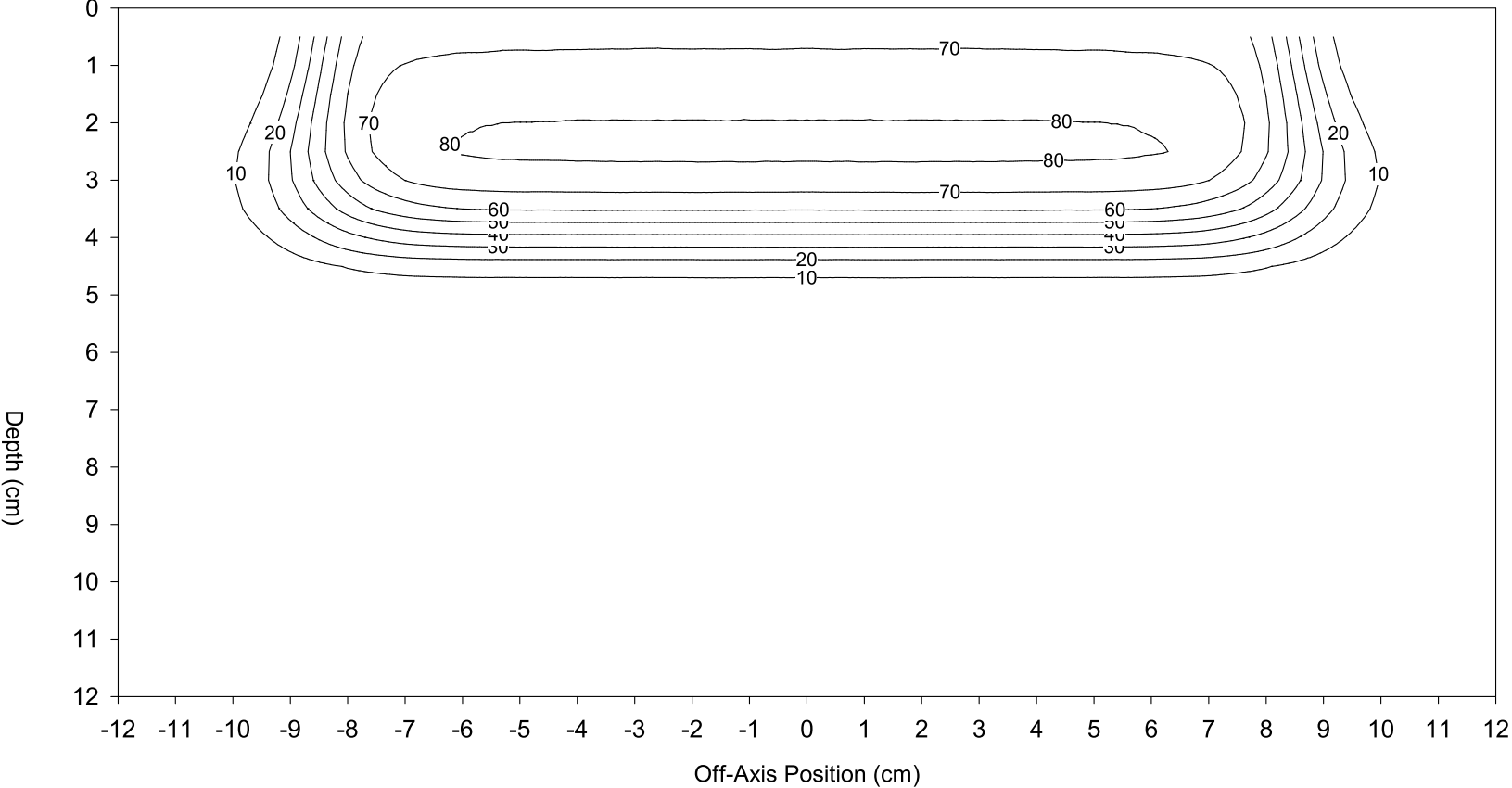
Configuration 2 - 9 MeV, Water, 110-cm SSD
