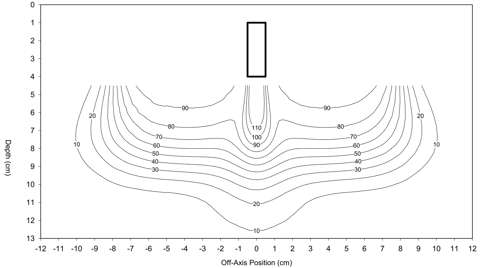
Configuration 7 - 20 MeV, Vertical Air Slab, 100-cm SSD
