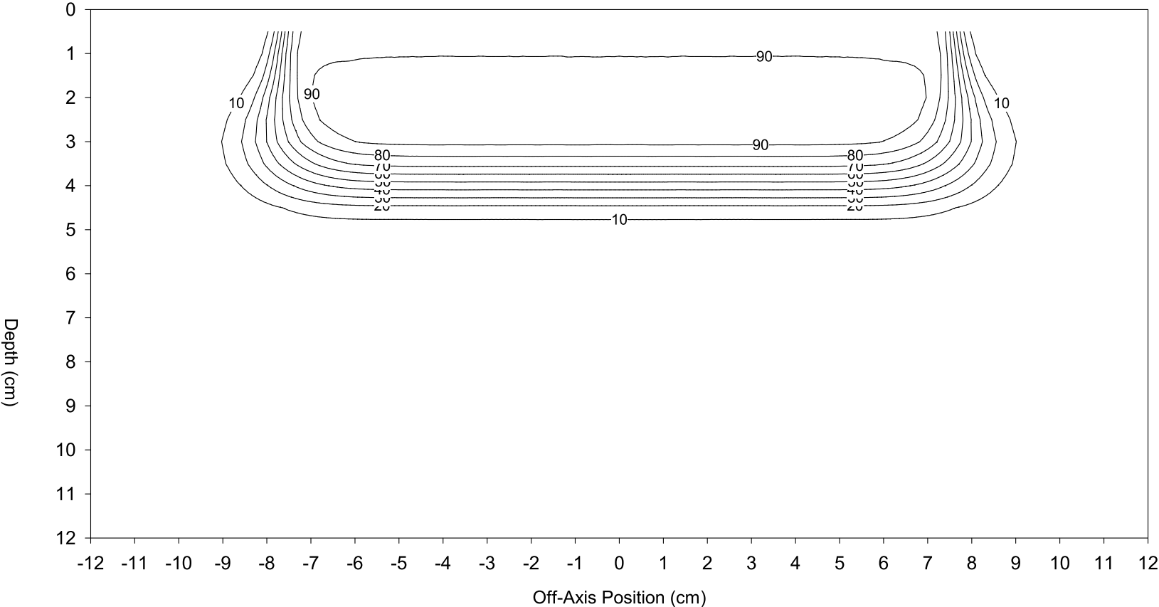
Configuration 1 - 9 MeV, Water, 100-cm SSD
